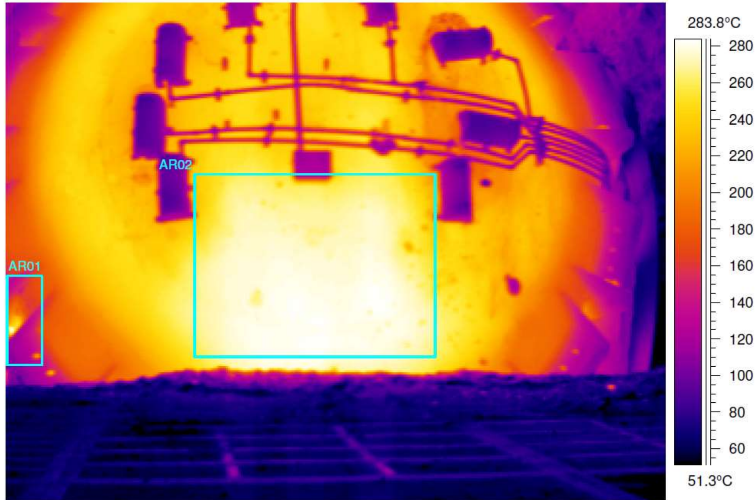
Thermography of BOS Vessel Shell
